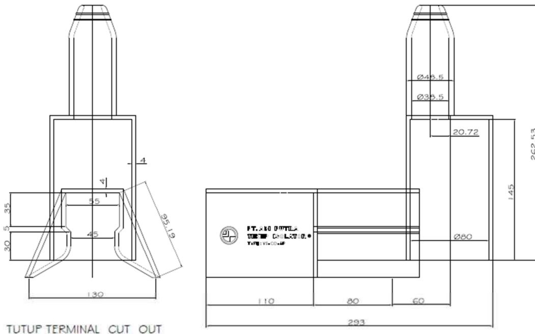
DIMENSI TEKEP ISOLATOR BUSHING/TEKEP ISOLATOR ARRESTER
