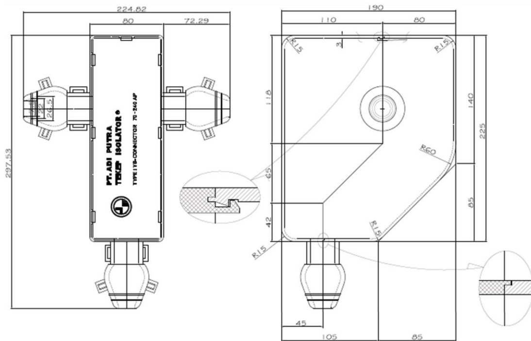
GAMBAR 1. DIMENSI TEKEP ISOLATOR CONNECTOR LLC
