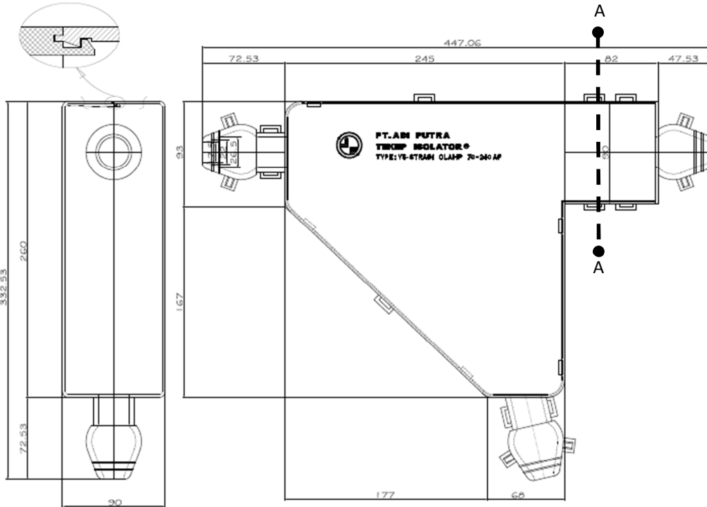
DIMENSI TEKEP ISOLATOR STRAINCLAMP/ TEKEP ISOLATOR CONNECTOR CCO
